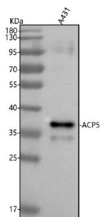
Figure 1. Western blot analysis of ACP5 using anti-ACP5 antibody (M03277-1).
